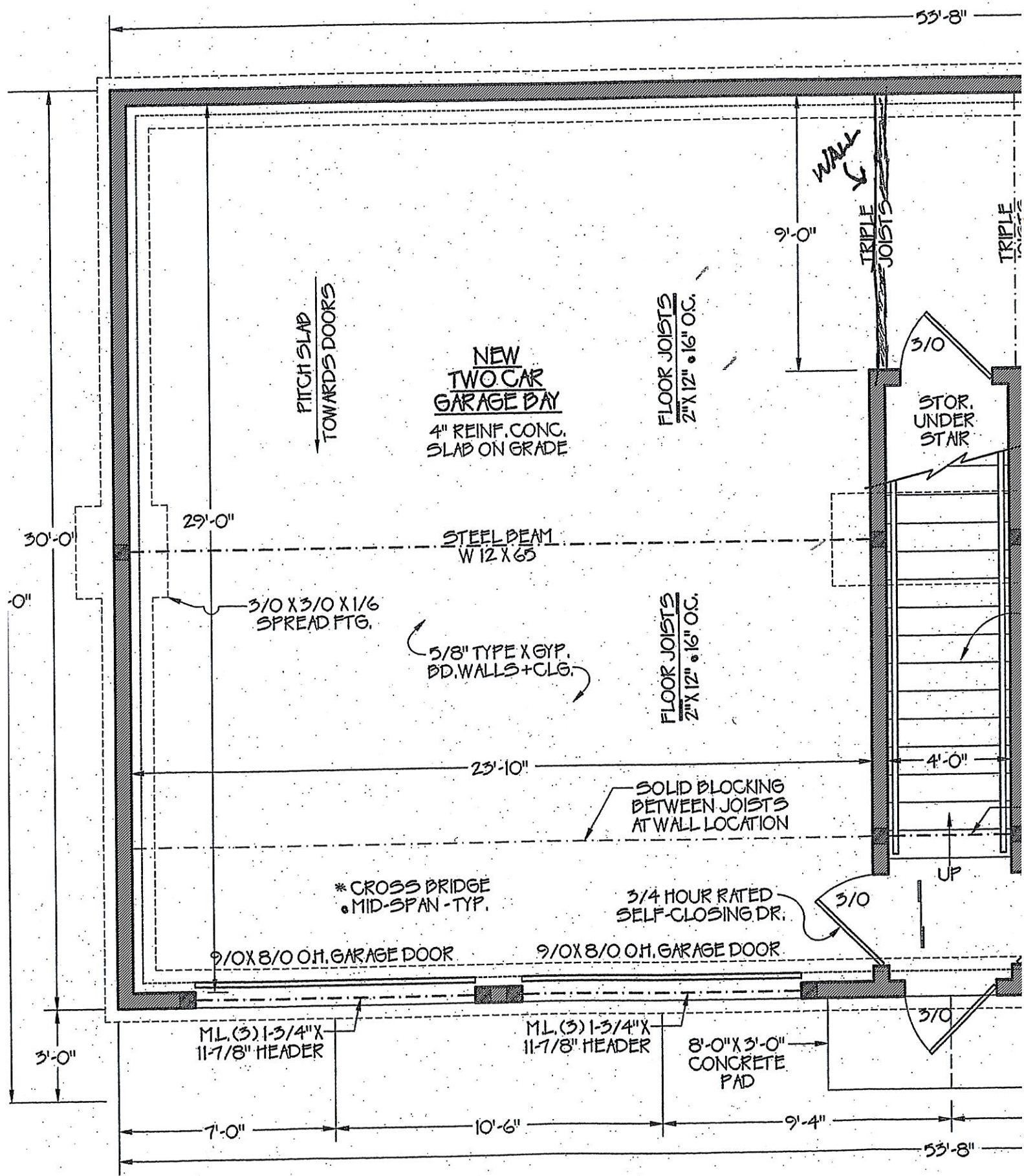
GARAGE FLOOR
